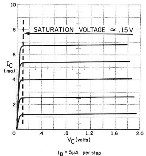
Figure 23. Saturation Voltage
