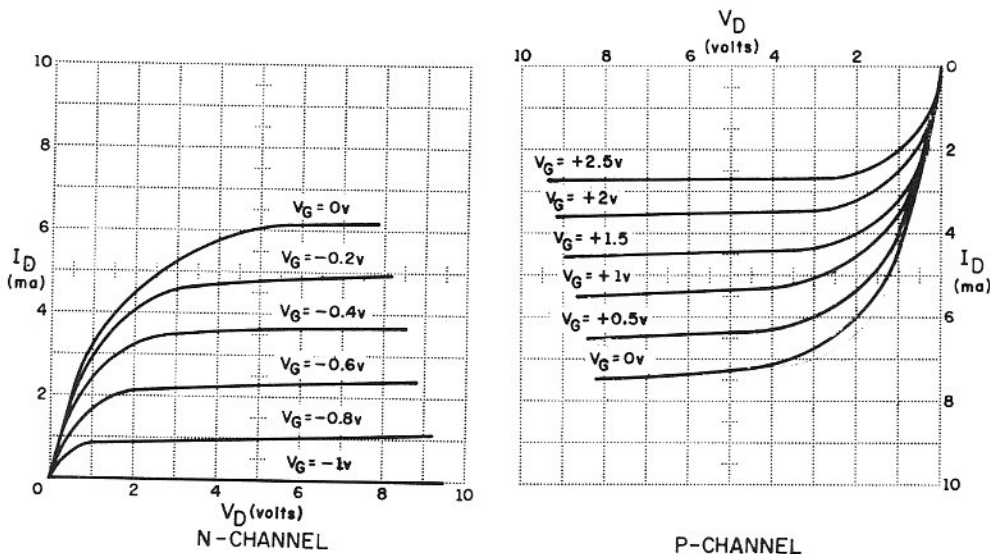
Figure 26. Typical FET Characteristic Curves
