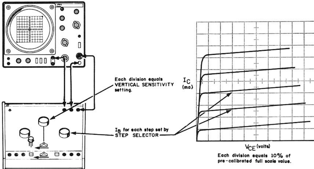
Figure 10. Typical Test of an NPN Transistor
