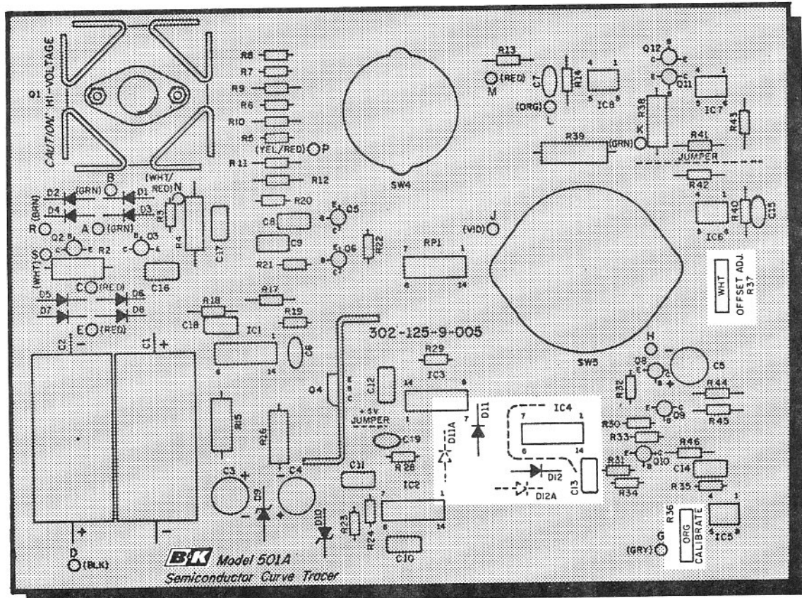
Figure 39. Curve Display Modification Diode Location
